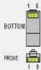
8 pin RJ45 (8P8C) male connector at the cables
